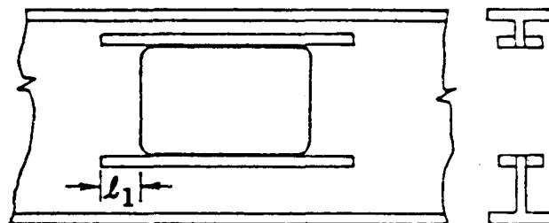
Fig. 5.7. Reinforced opening.
