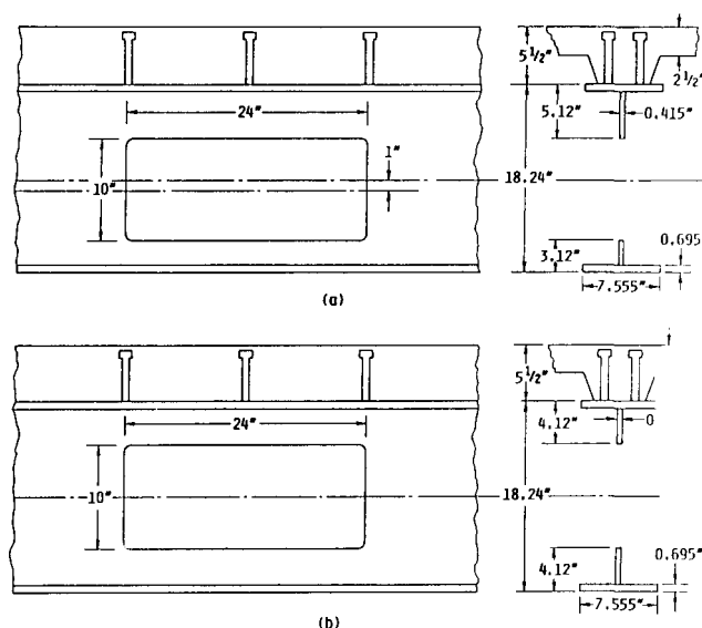
Fig. 4.12. Details for Example 4. (a) Eccentric opening, (b) concentric opening.
